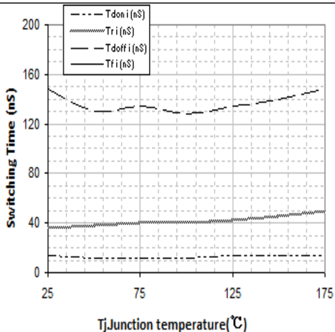
Switching Time vs. Tj
